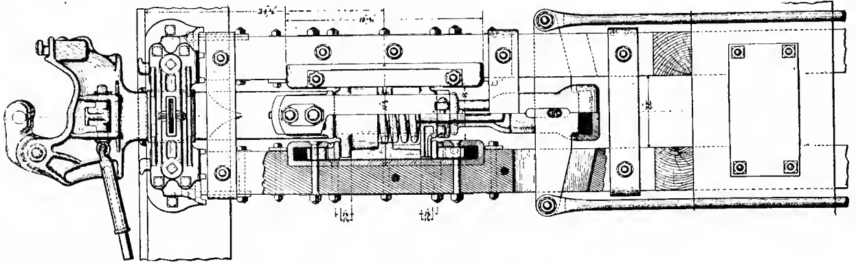
Fig. 2276. Sectional Plan.
